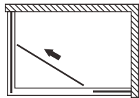
HS-002 SIZE: 1200 X 800 X 2000 mm 1200 X 900 X 2000 mm
