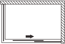
JL-003+JL004 SIZE: 1000 X 700 X 1850 mm 1200 X 800 X 1850 mm 1400 X 900 X 1850 mm
